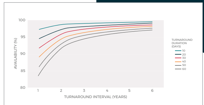
Figure 1: Availability loss due to turnarounds by duration & interval
